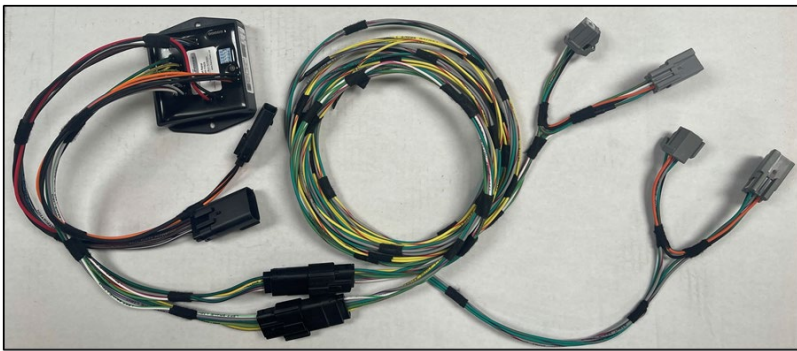
Black-Out Module w/ Utility Harness
