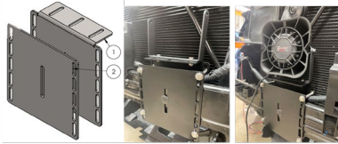
UNISPBRKT, Universal No-Drill Speaker Mounting Bracket
