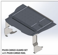
PIU20-CARGO-GUARD-SET with PIU20-CARGO-RAIL
